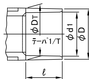
(呼び径65~150mm)
